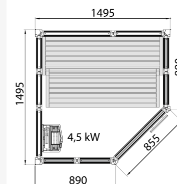
IMPRESSION SAUNA i1515/C
