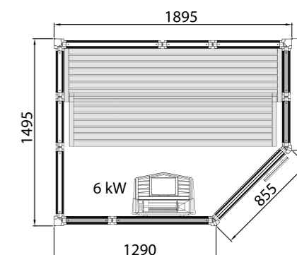
IMPRESSION SAUNA i1915/C
