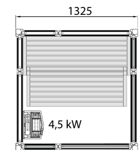
IMPRESSION SAUNA i1313
